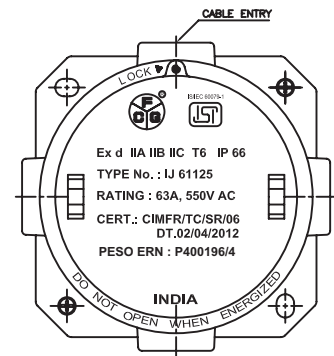
FIG-3 (4 WAY)
