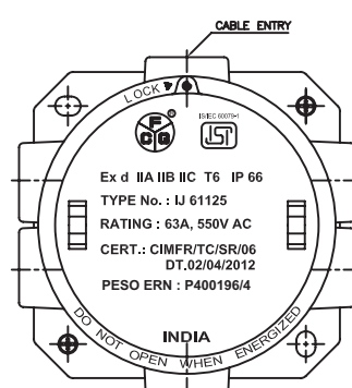
FIG-2 (6 WAY)
