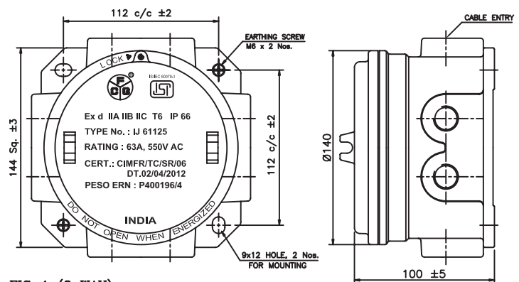
FIG-1 (8 WAY)
