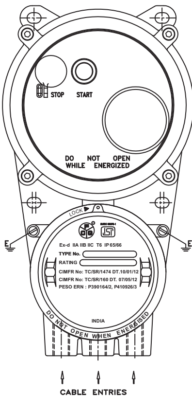
WITHOUT ISOLATOR
