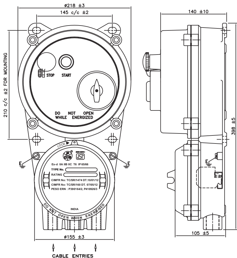
WITH ISOLATOR
